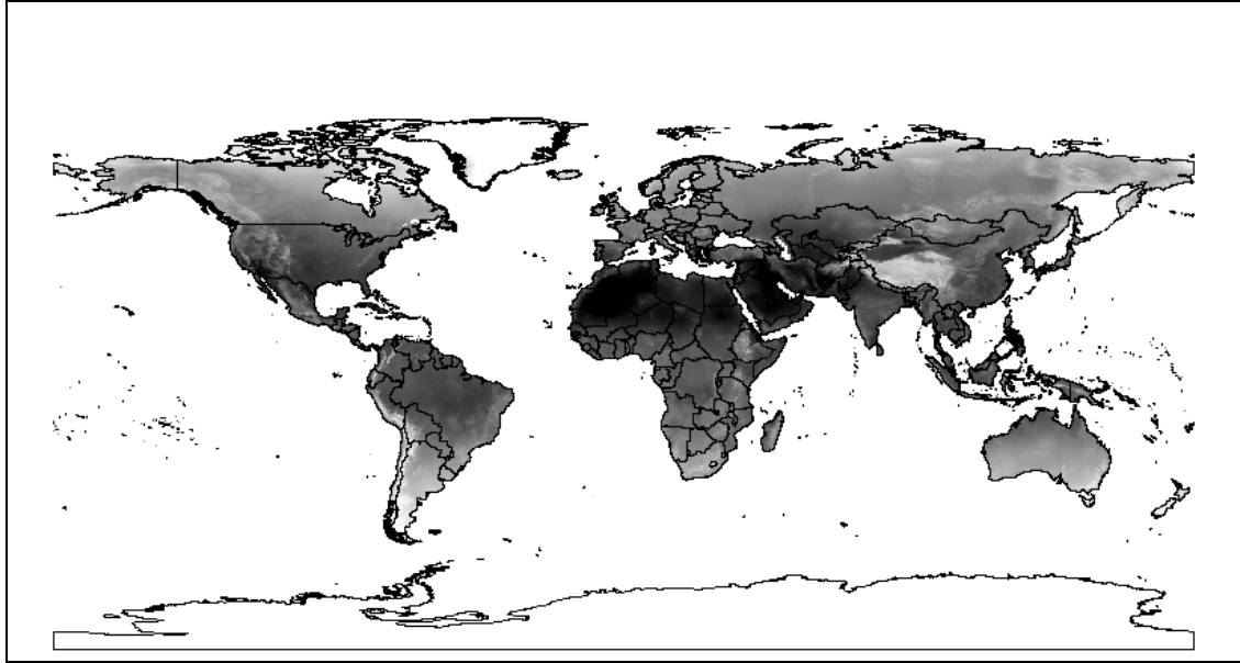
Figure 12. Global Raster Image for Maximum Temperature During July
