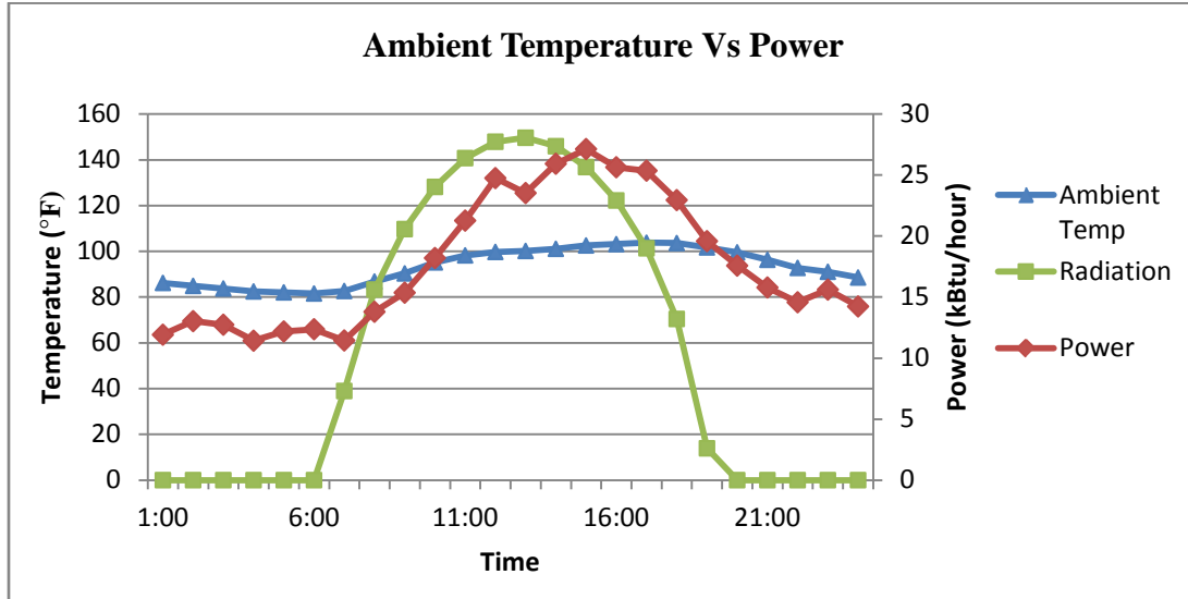
Figure 4. Graphic Data From Shelter Tests (AFCESA, 2011)
